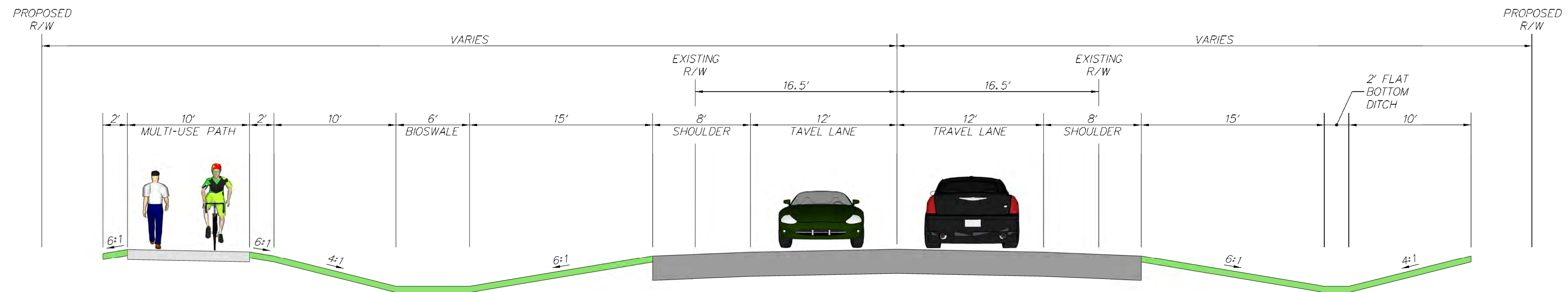
OPEN DRAINAGE SECTION
