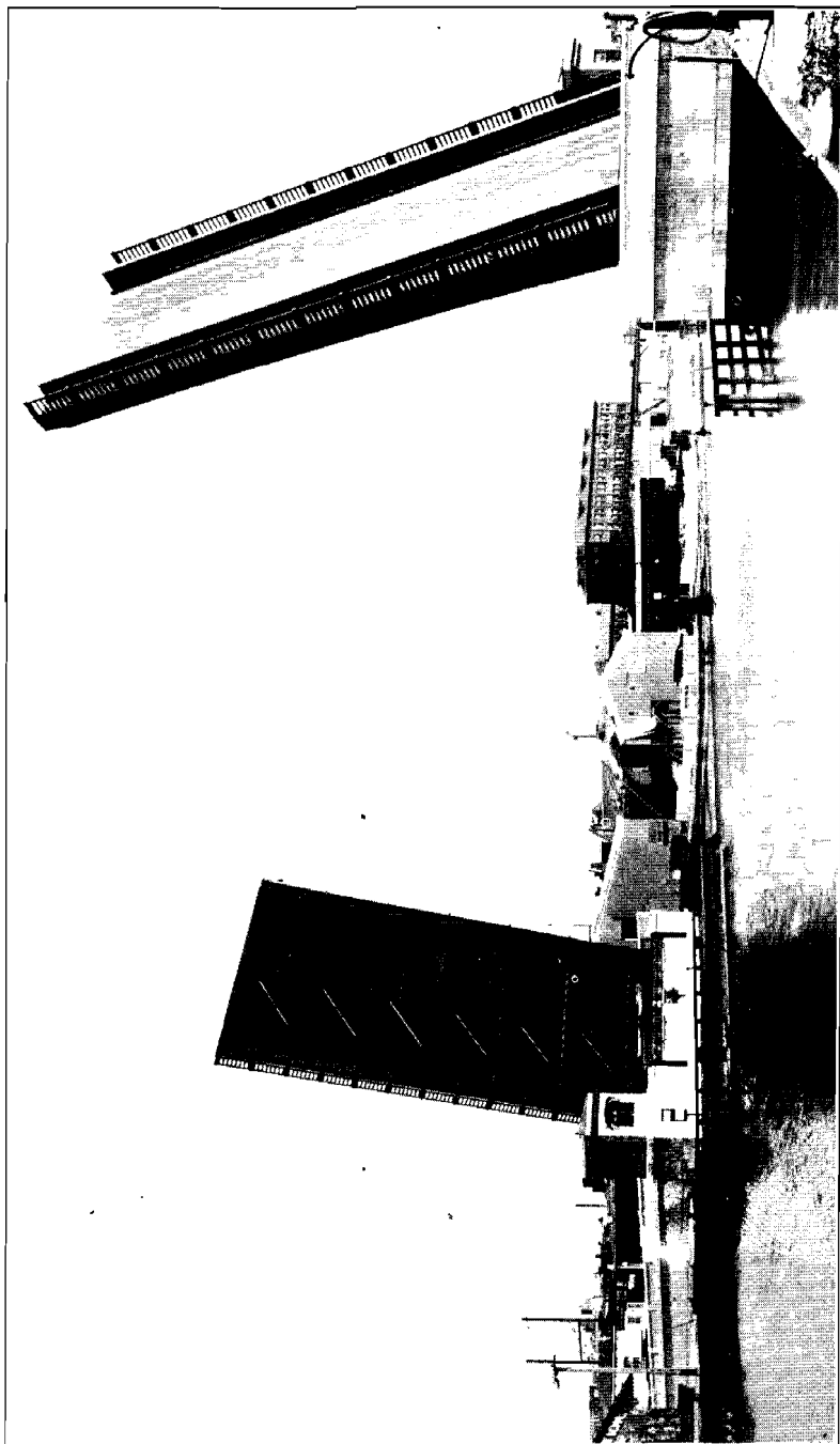
SOUTH MARKET STREET BRIDGE, WILMINGTON, DOUBLE LEAF TRUNION TYPE BASCULE. COMPLETED 1927.
