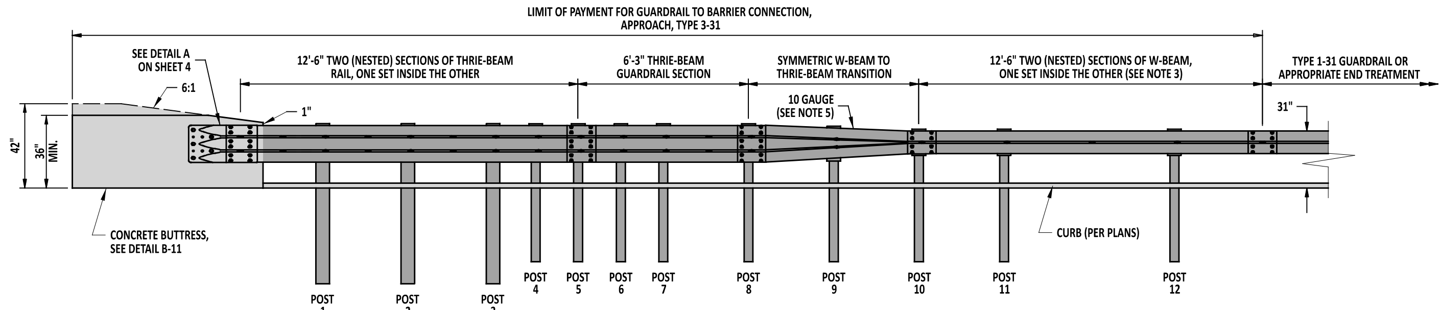
ELEVATION VIEW
