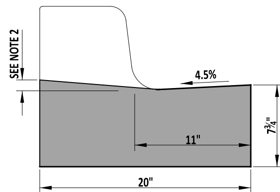
INTEGRAL PCC CURB AND GUTTER TYPES 3-2 THRU 3-8
