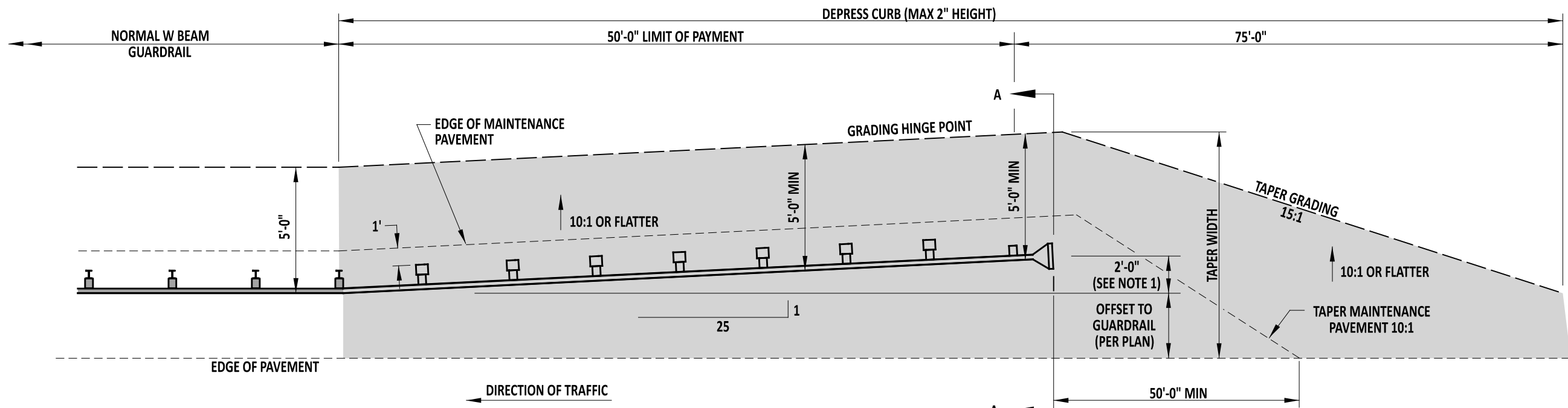
PLAN VIEW
