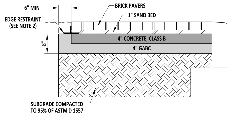
BRICK PAVER SIDEWALK DETAIL
