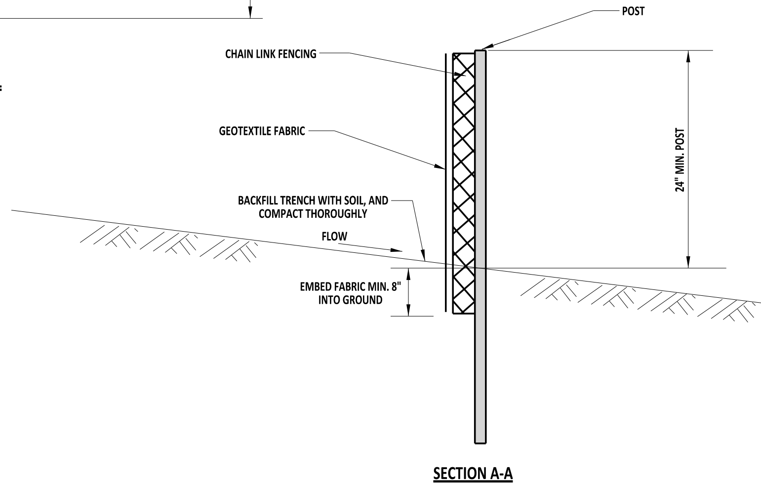
SUPER SILT FENCE CONSTRUCTION DETAIL
