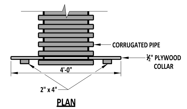
ANTI-SEEP COLLAR
