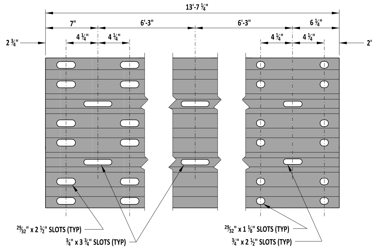
THRIE BEAM EXPANSION ELEMENT
