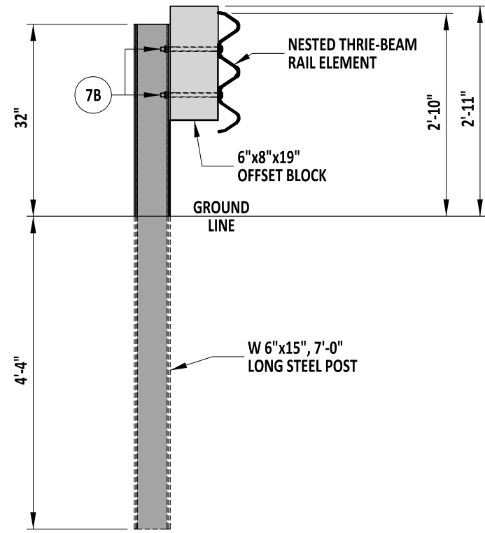
SECTION POSTS 1-3
