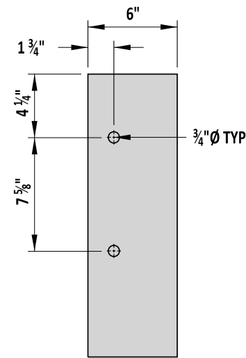
ELEVATION VIEW OFFSET BLOCK FOR POSTS 1-3
