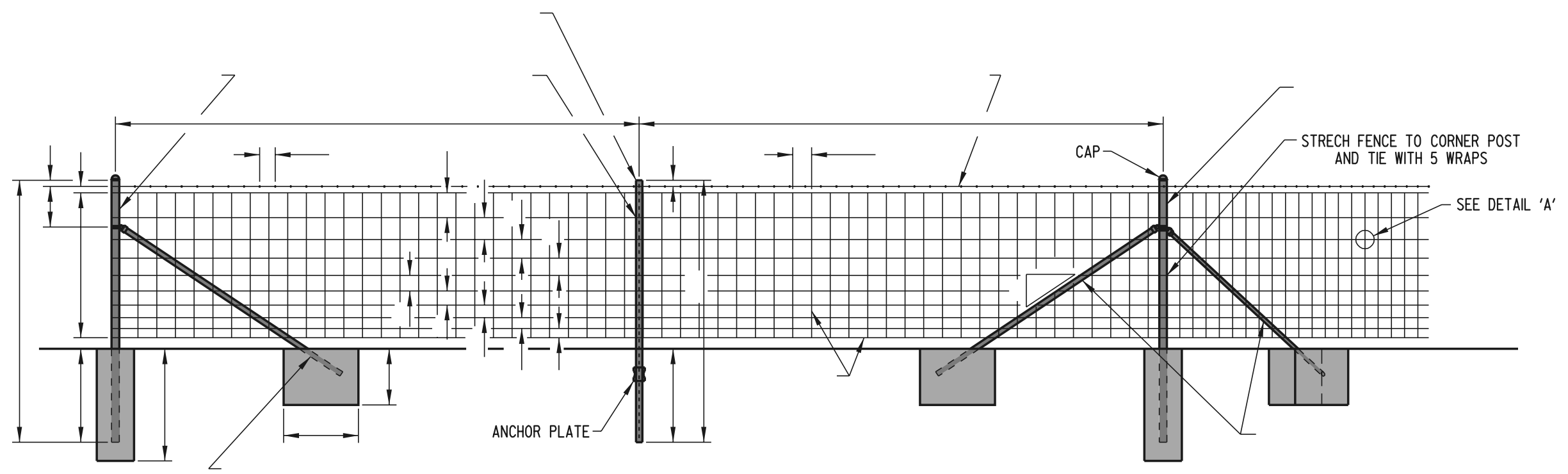
FRONT VIEW
