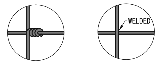
DETAILED 'A'
