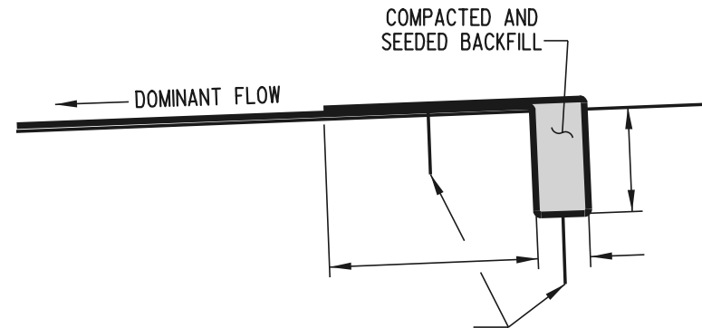
TERMINAL TRENCH ANCHOR DETAIL
