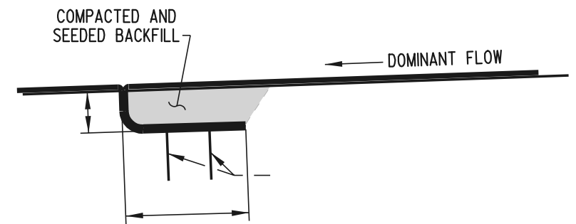
OVERLAP DETAIL
