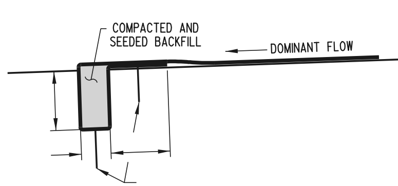
INITIAL TRENCH ANCHOR DETAIL
