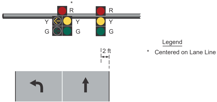
Figure IV-5a. One Through Lane with One Left-Turn Lane (Protected-Permissive Left-Turn Phasing)
