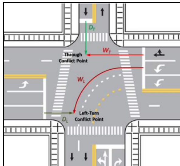
Figure IV-9. Intersection Conflict Points
