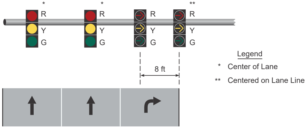
Figure IV-5m. Two Through Lanes With One Right-Turn Lane (Protected-Only Right-Turn Phasing)
