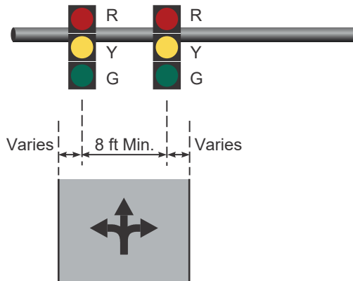
Figure IV-5n. One Shared Left/Through/Right Lane (Permissive Left-Turn Phasing)
