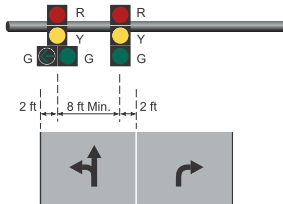
Figure IV-6e. One Shared Left/Through Lane and One Right-Turn Lane (Split Phasing)
