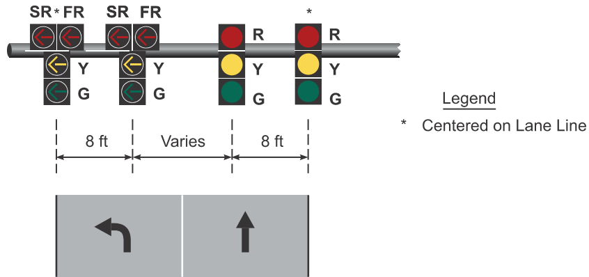
Figure IV-5b. One Through Lane with One Left-Turn Lane (Protected-Permissive Left-Turn Phasing FRA)
