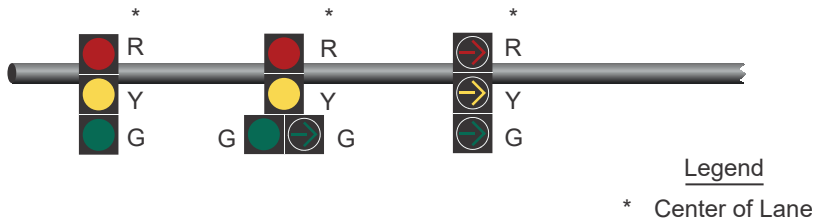
Figure IV-5j. Two Through Lanes With One Right-Turn Lane (Permissive Right-Turn Phasing)
