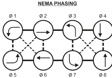
Figure IV-7. Standard NEMA Phasing Convention
