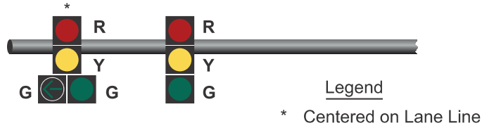
Figure IV-6c. One Left-Turn Lane, One Shared Left/Through Lane, One Through Lane, and One Right-Turn Lane (Split Phasing)
