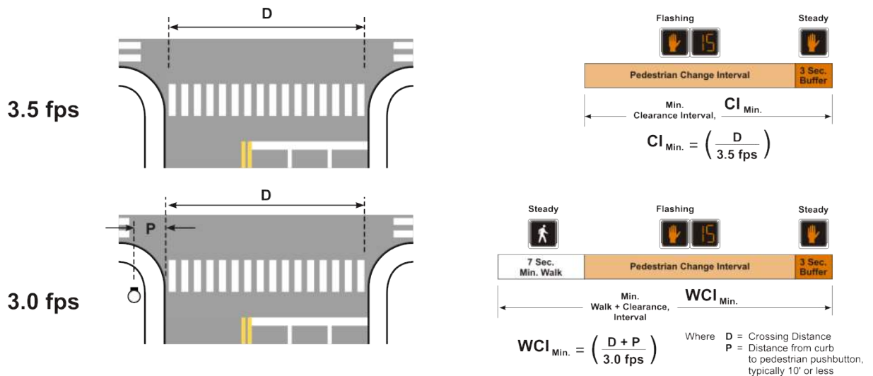
Figure IV-14. Clearance Interval Time Calculations
