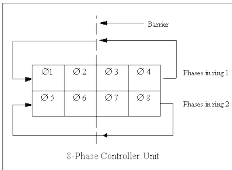
Figure IV-12. Sequence of Phases for Dual-Ring 8-Phase Controller Unit
