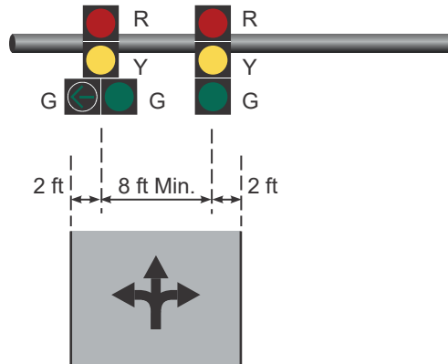
Figure IV-6f. One Shared Left/Through/Right Lane (Split Phasing)
