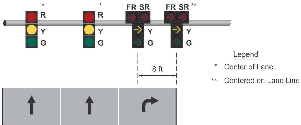
Figure IV-5l. Two Through Lanes with One Right-Turn Lane (Protected-Permissive Right-Turn Phasing FRA)
