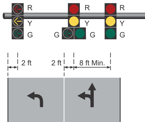
Figure IV-6a. One Left-Turn Lane with One Shared Left/Through Lane (Split Phasing)
