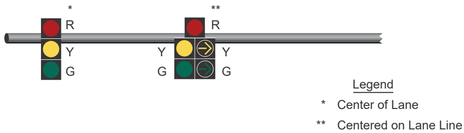
Figure IV-5h. Three Through Lanes with Two Left-Turn Lanes (Protected-Only Left-Turn Phasing)
