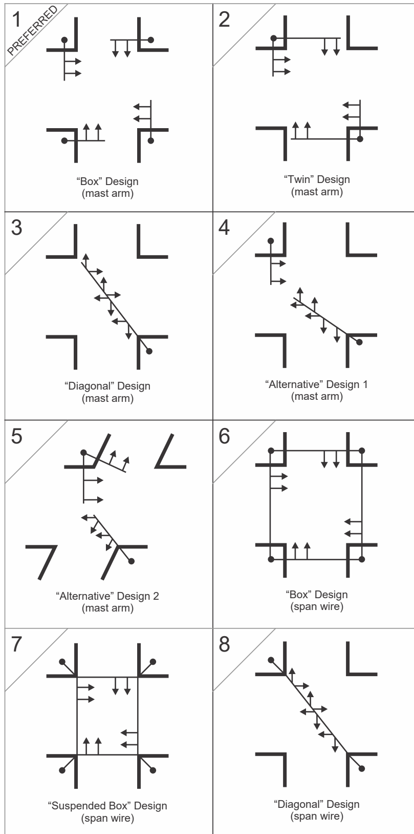
Figure IV-2. Typical Layouts of Signal Poles and Signal Heads
