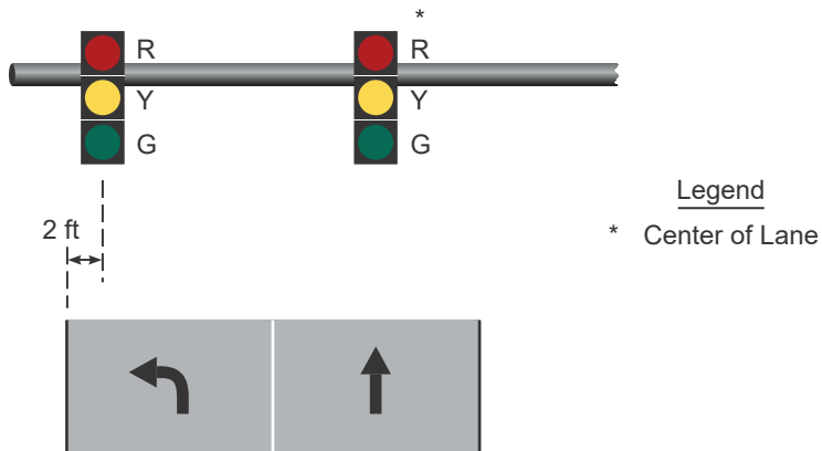
Figure IV-5o. One Left-Turn Lane With One Through Lane (Permissive Left-Turn Phasing)
