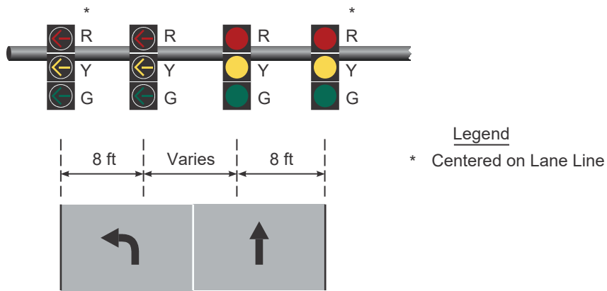
Figure IV-5c. One Through Lane with One Left-Turn Lane (Protected-Only Left-Turn Phasing)
