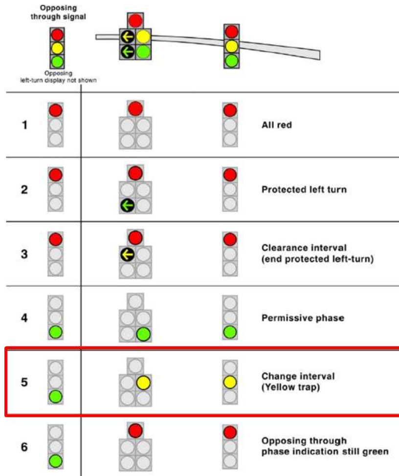
Figure IV-11. Yellow Trap with Protected/Permissive Left-Turn Phasing
