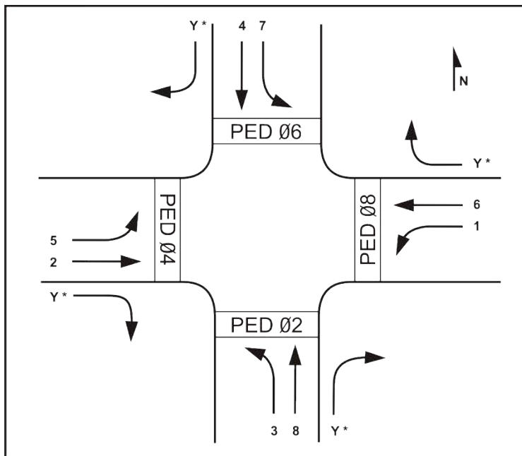
Figure IV-8. Typical Intersection Movements and Corresponding NEMA Phasing Convention
