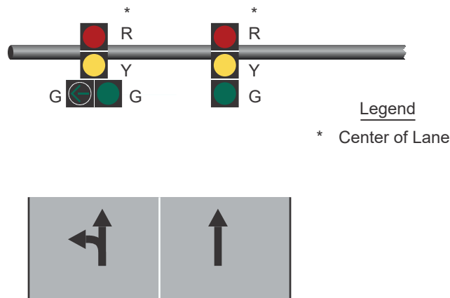
Figure IV-6b. One Shared Left/Through Lane With One Through Lane (Split Phasing)
