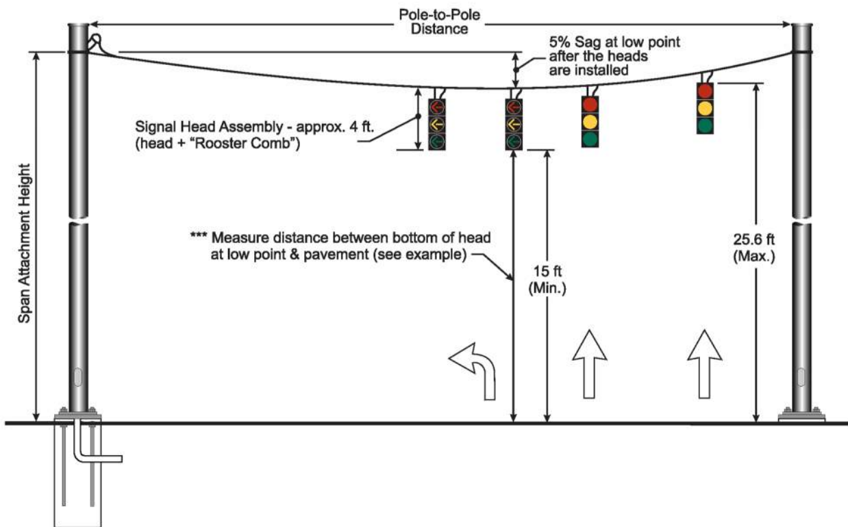
Figure IV-1. Sag Calculation
