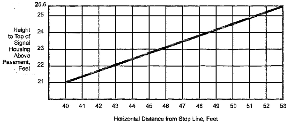
Figure IV-4. Maximum Mounting Height of Signal Housings
