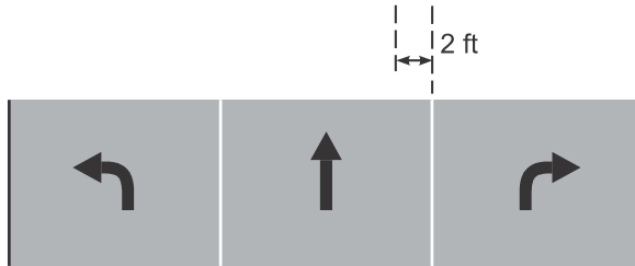
Figure IV-6d. One Left-Turn Lane, One Through Lane, and One Right-Turn Lane (Split Phasing)
